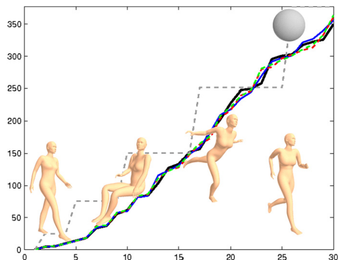
Fig. 9. First 30 eigenvalues plotted for the girl in four different postures as opposed to the spectrum of the sphere (gray) with same surface area (the position of the shapes in the plot is irrelevant).
